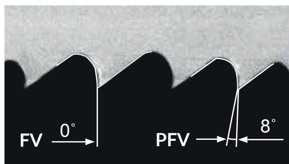
PFV 8° in variable tooth pitches 2/3, 3/4, 4/6 and 5/8 FV: 0° in variable tooth pitches 6/10, 8/12 and 10/14
